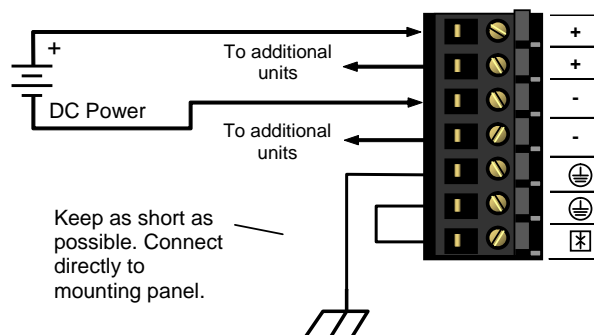
Figure 4: Field Wiring
