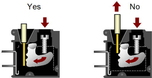
Figure 6: Terminal Connection
