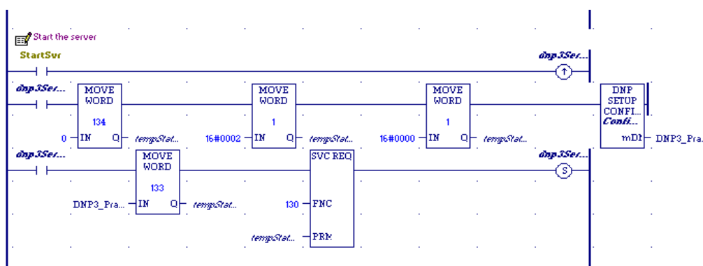
Figure 21: START Service Request
