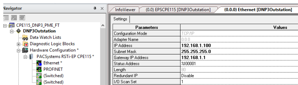
Figure 10: Configuring the Ethernet IP Address CPE115
