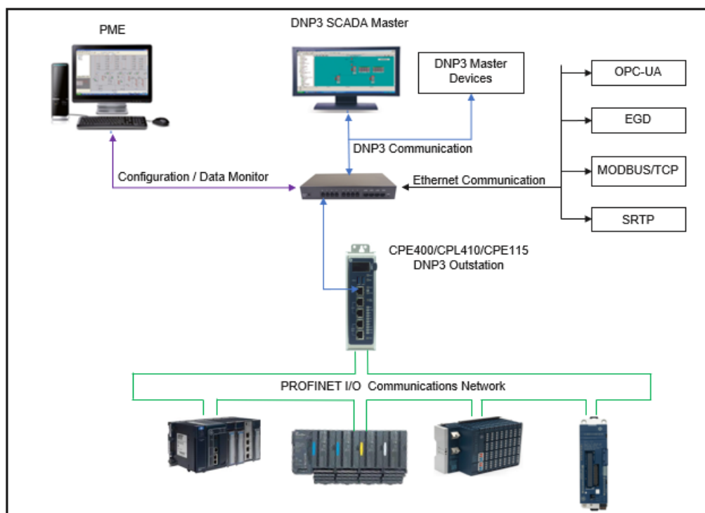
Figure 3: Application Showing CPE400/CPL410/CPE115 with DNP3 Outstation - Simplex System Overview
