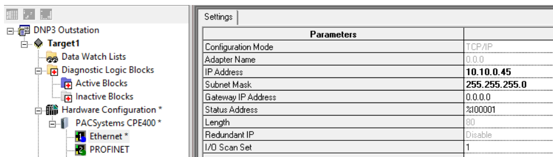
Figure 9: Configuring the Ethernet IP Address
