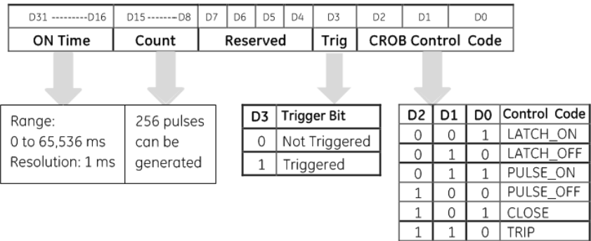
Figure 14: CROB Control DWord Layout
