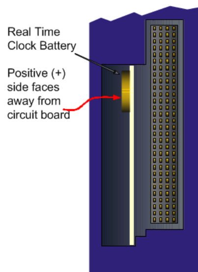
Figure 17: Accessing Real-Time Clock Battery (CPE302-Axxx, CPE305-Axxx, and CPE310-Axxx)
