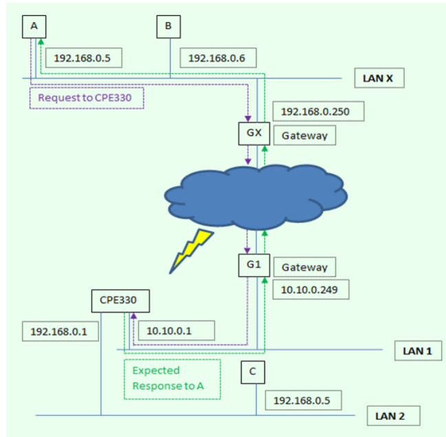
Figure 48: Expected Response Path
