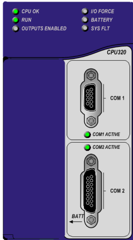
Figure 22: IC695CPU320 Front View
