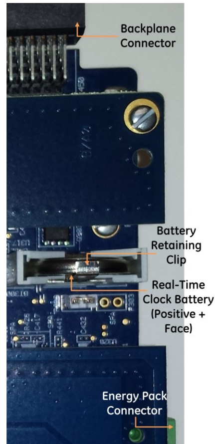
Figure 11: Location and Orientation of Real-Time Clock Battery in CPE330
