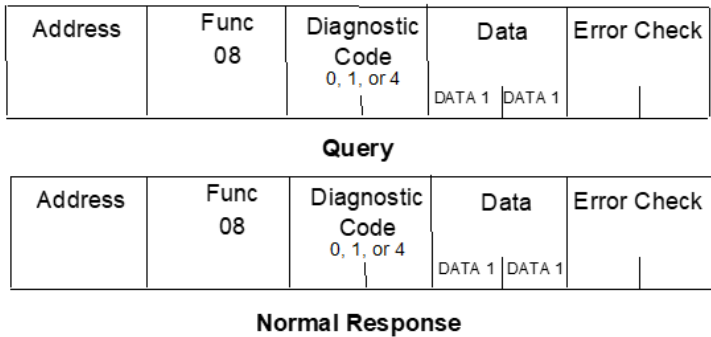
Figure 63: RTU Loopback/Maintenance Message Format
