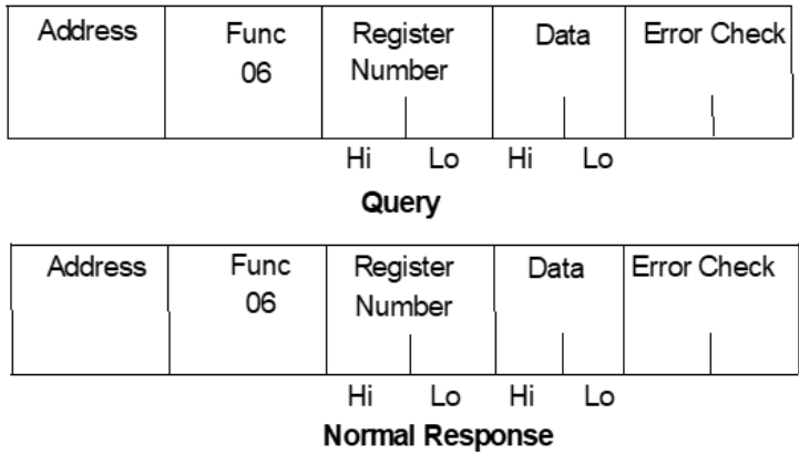
Figure 61: RTU Preset Single Register Message Format
