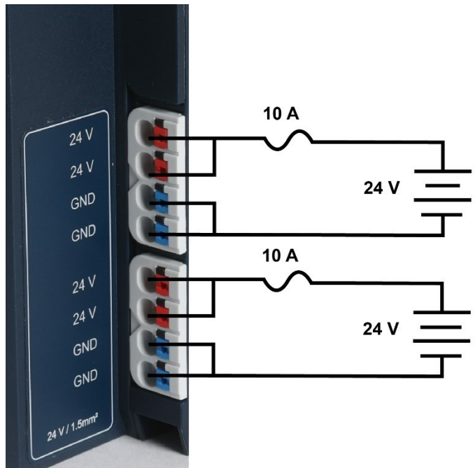
Figure 33: Power Feed Maximum Current Draw
