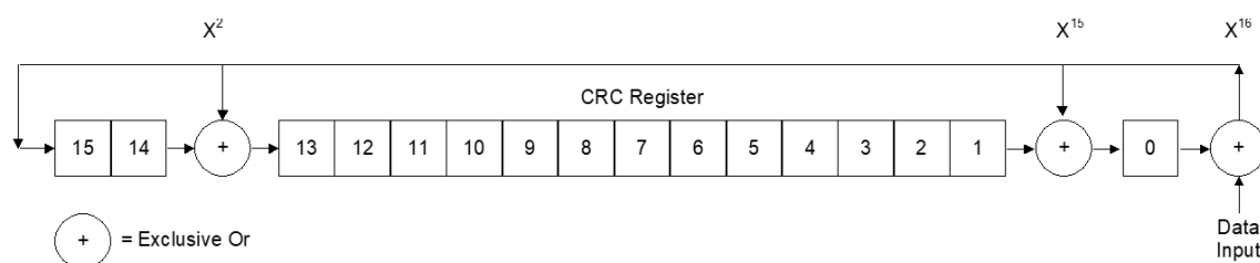
Figure 55: CRC Register Operation
