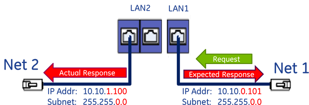
Figure 47: CPE330 Overlapping Local IP Subnet Example
