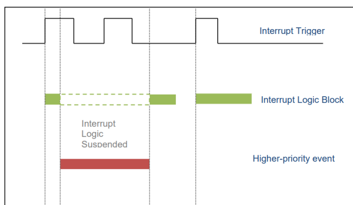
Figure 69: Interrupt Execution Considerations
