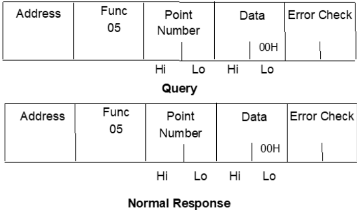
Figure 60: RTU Force Single Output Message Format
