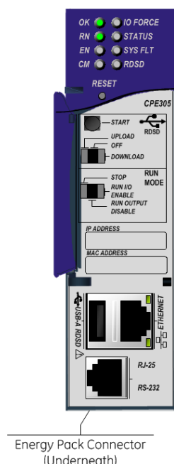
Figure 15: External Features of CPE302/CPE305-Axxx
