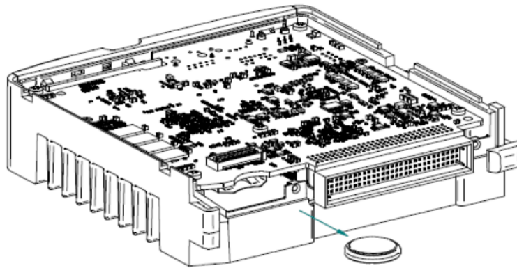
Figure 20: Use Tweezers to Remove Battery
