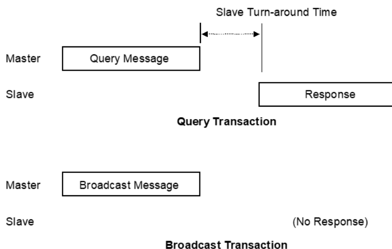
Figure 52: RTU Message Transactions
