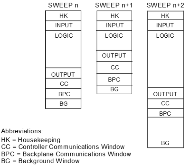
Figure 42: Typical Sweeps in Normal Sweep Mode
