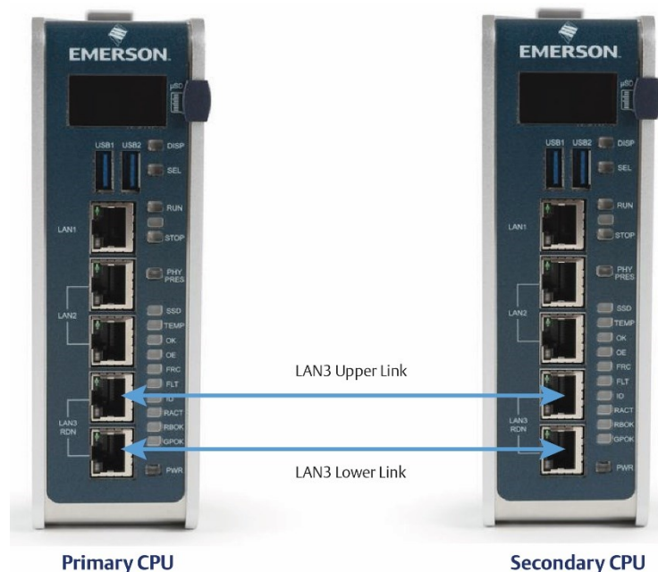
Figure 7: LAN3 Interconnects for Hot Standby Redundancy
