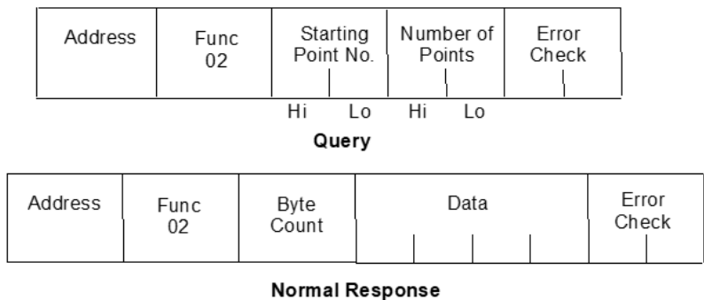
Figure 57: RTU Read Input Table Message Format
