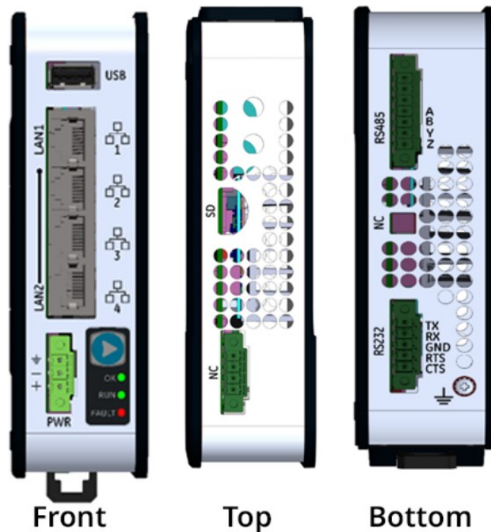
Figure 24: CPE100 Front, Top, and Bottom Views and Features
