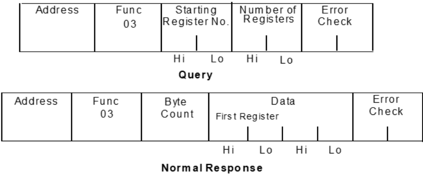
Figure 58: RTU Read Registers Message Format
