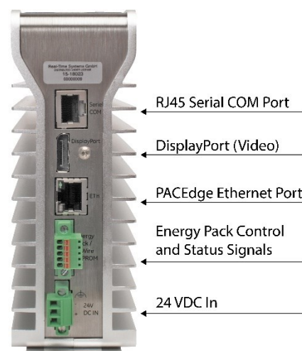
Figure 4: Underside Ports & Connectors
