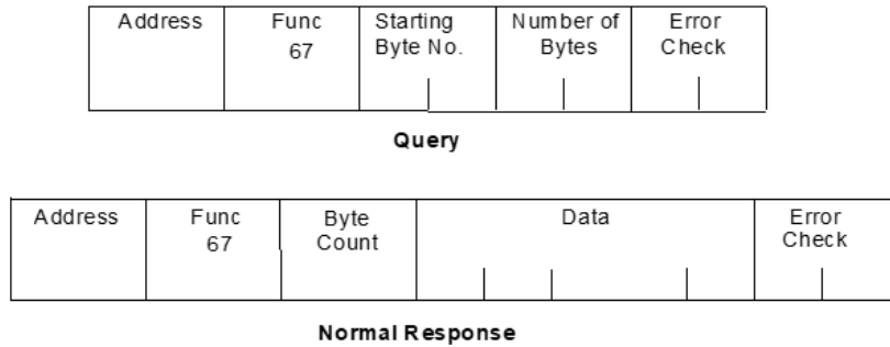
Figure 67: RTU Read Scratch Pad Memory Message Format
