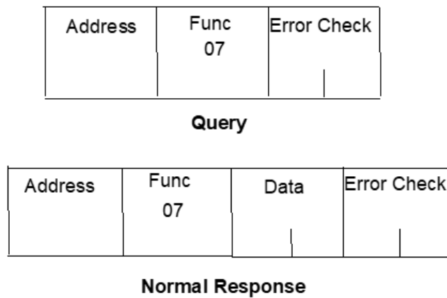
Figure 62: RTU Read Exception Status Message Format
