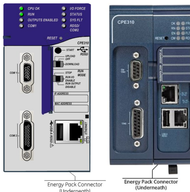
Figure 16: External Features of CPE310-Axxx/Bxxx
