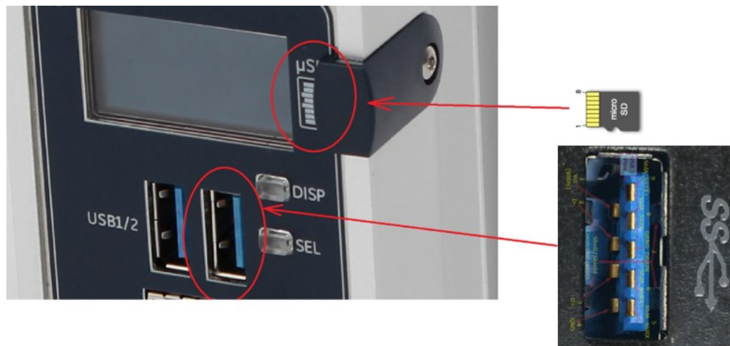
Figure 5: CPE400 Micro-SD & USB Connectors
