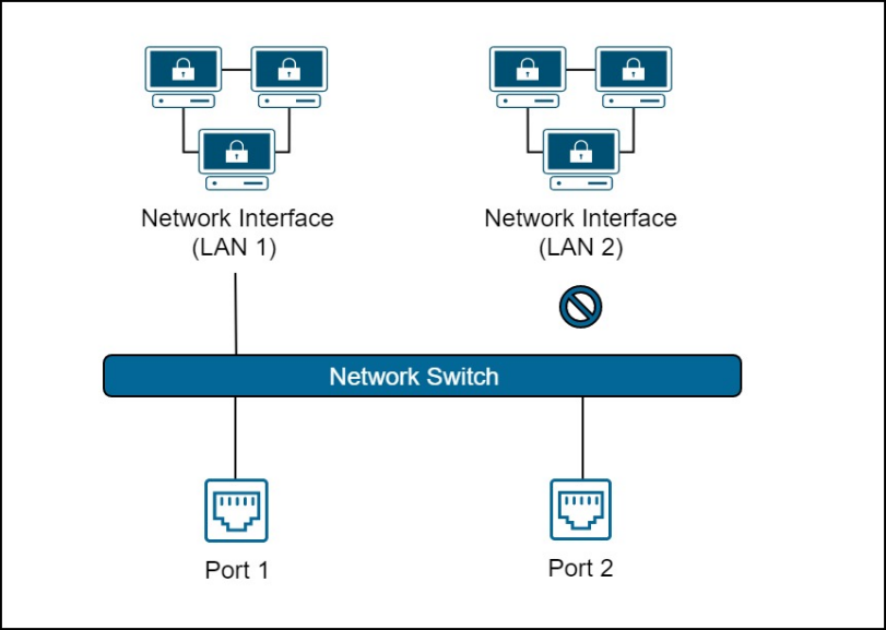
Figure 35: Single-LAN Mode
