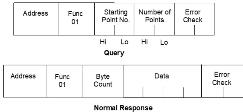
Figure 56: RTU Read Output Table Message Format
