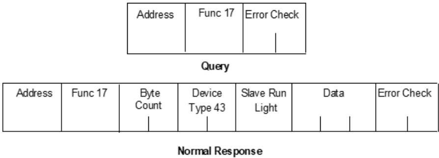
Figure 66: RTU Report Device Type Message Format
