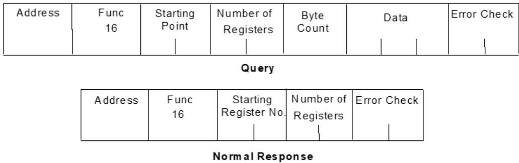
Figure 65: RTU Preset Multiple Registers Message Format
