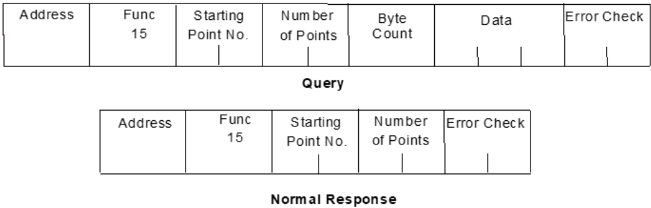
Figure 64: RTU Force Multiple Outputs Message Format
