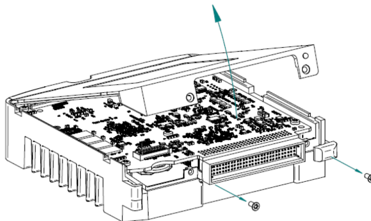
Figure 19: Remove Screws Before Opening Cover
