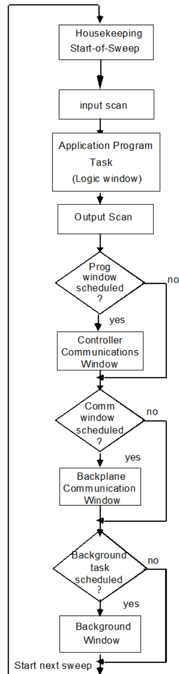
Figure 41: Major Phases of a Typical CPU Sweep
