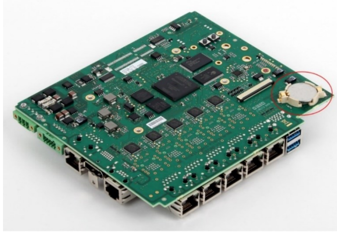
Figure 6: Location of RTC Battery on CPE400/CPL410
