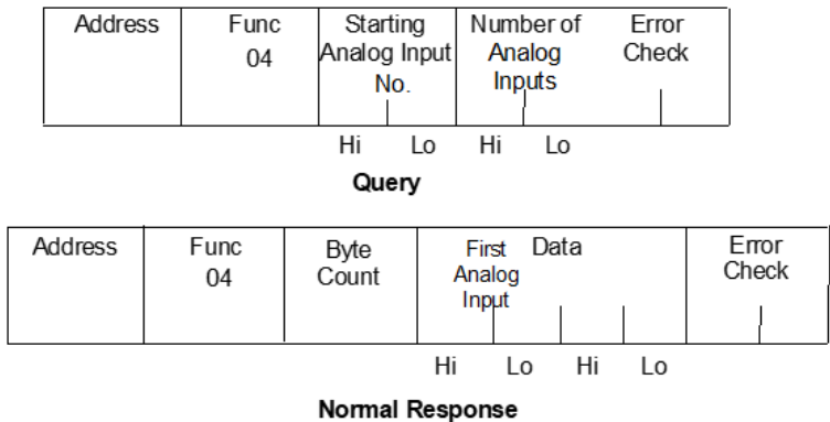
Figure 59: RTU Read Analog Inputs Message Format
