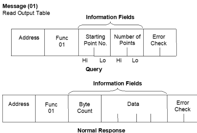
Figure 54: RTU Read Output Table Example
