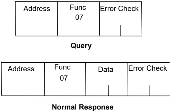
Figure 59: RTU Read Exception Status Message Format
