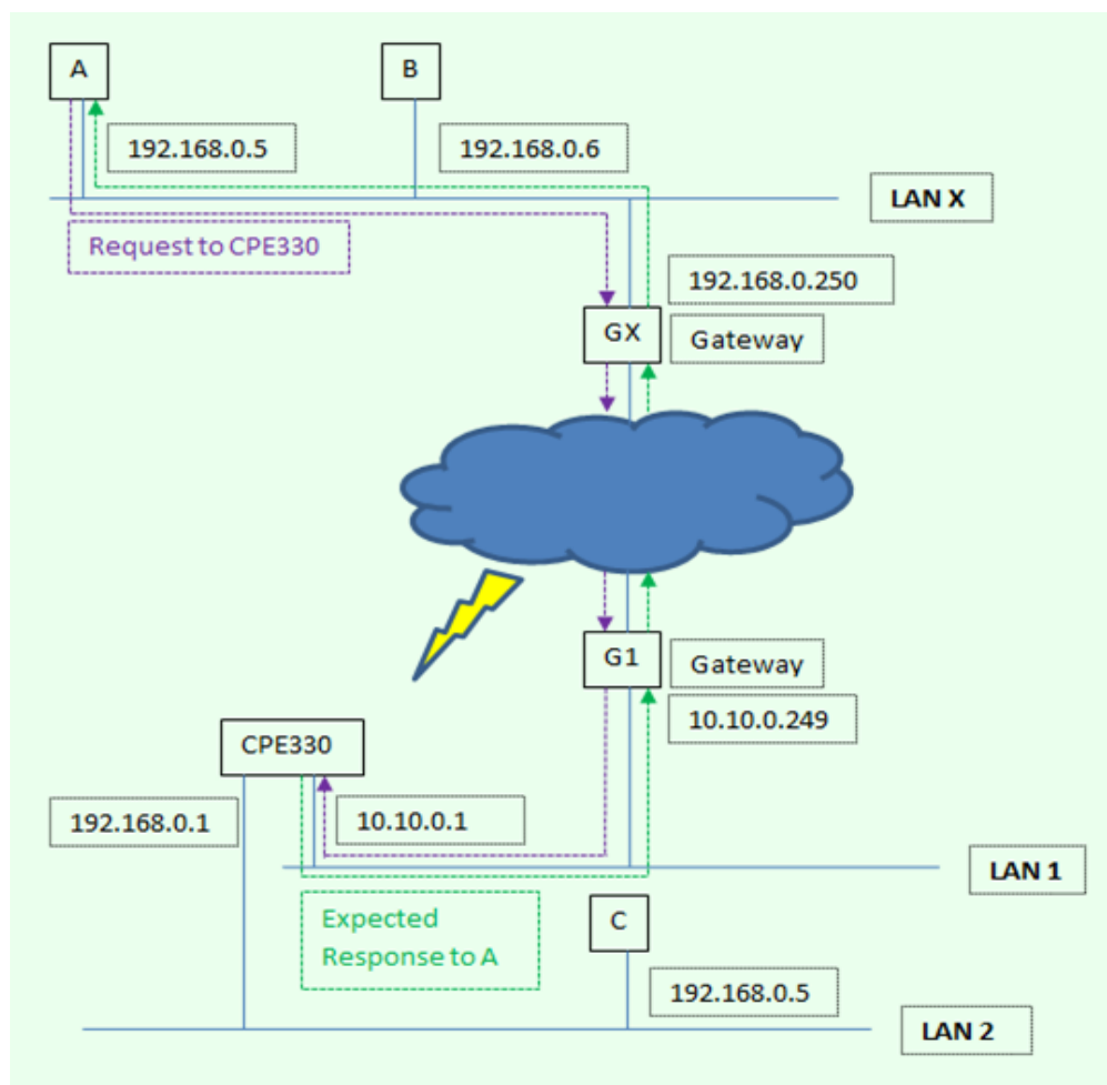
Figure 46: Expected Response Path
