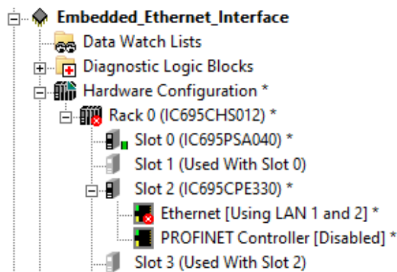
Figure 38: Embedded Ethernet Interface Configuration
