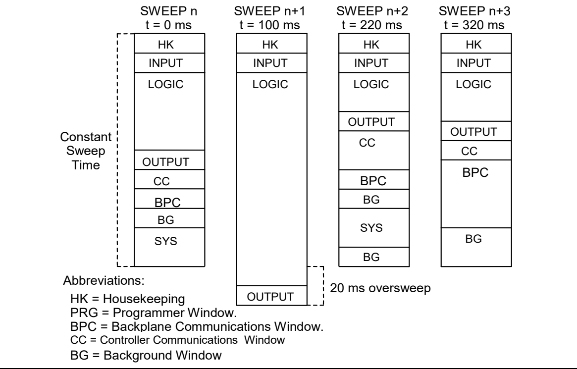
Figure 42: Typical Sweeps in Constant Sweep Mode
