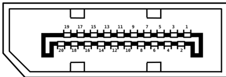
Figure 18: Display Port Connector
