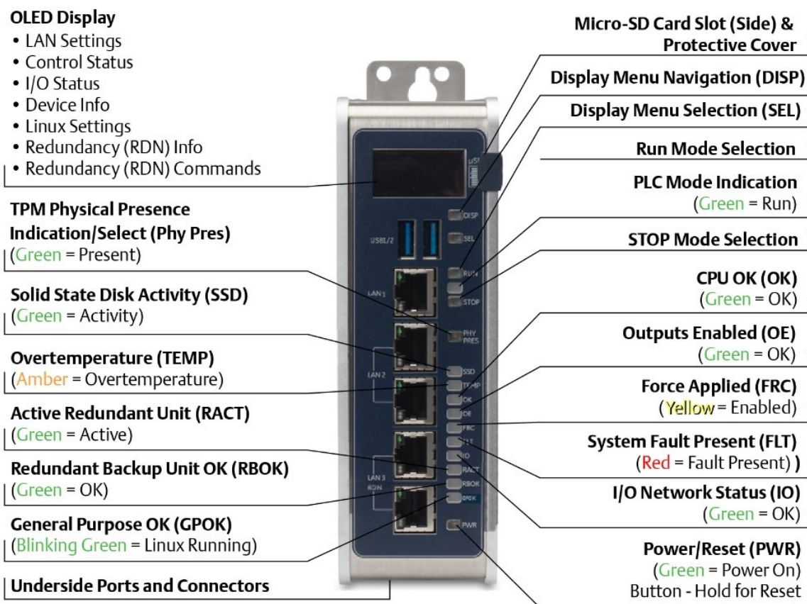
Figure 6: CPE400 Front View and Features
