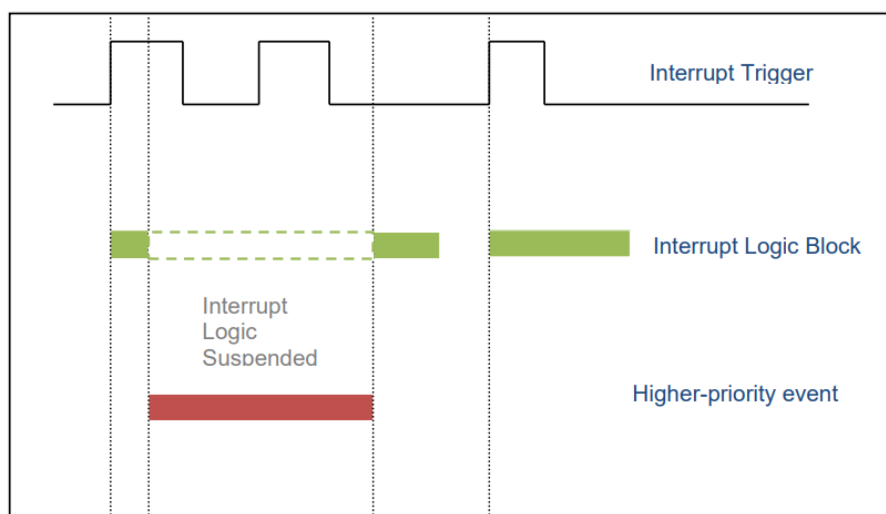
Figure 65: Interrupt Execution Considerations
