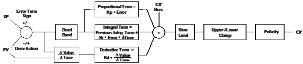
Figure 259: PID_IND Diagram
