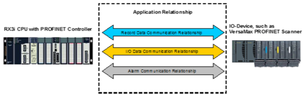
Figure 90: Application Relationship
