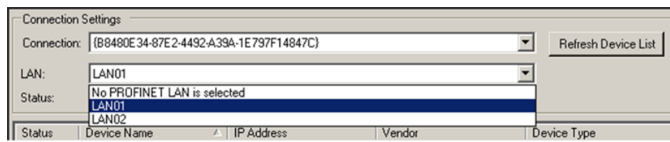
Figure 88: Assign LAN
