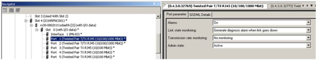
Figure 81: Editing Port Parameters on Third-Party I/O Device
