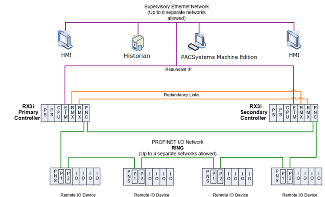
Figure 15: RX3i Hot Standby CPU Redundancy Network with MRP Ring Topology
