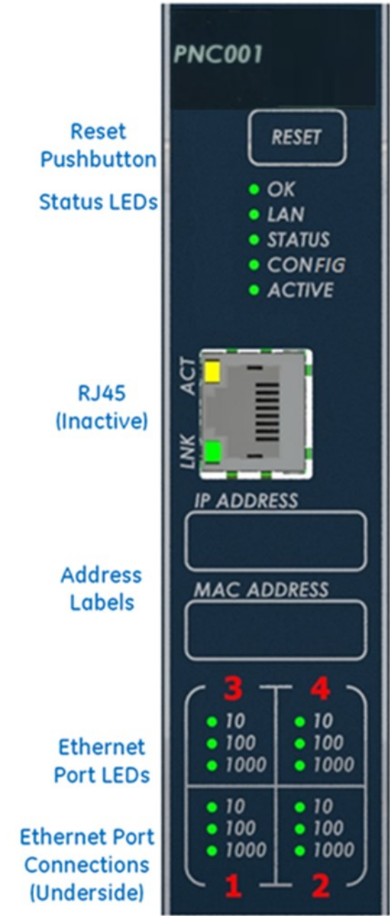
Figure 3: IC695PNC001-Bxxx Controls & Indicators
