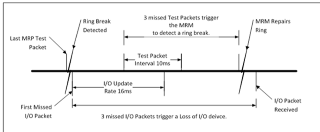
Figure 99: Timeline for Successful MRP Ring Repair at 16ms I/O Update Rate
