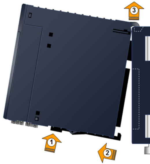
Figure 21: Remove Module from RX3i Backplane
