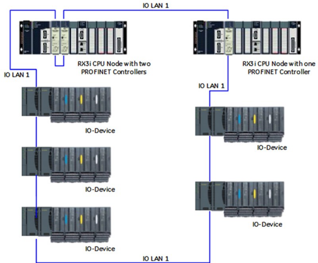
Figure 101: Ring Topology with Multiple Controllers
