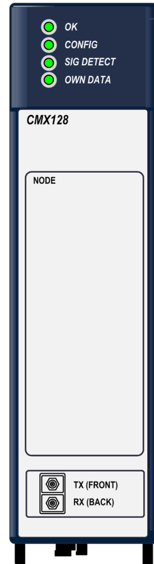
Figure 379: IC695CMX128
