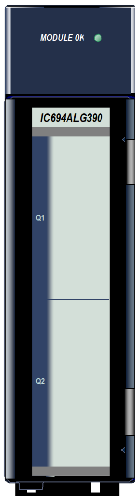
Figure 291: IC694ALG390
