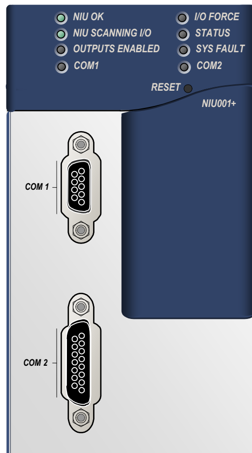
Figure 405: IC695NIU001 PLUS
