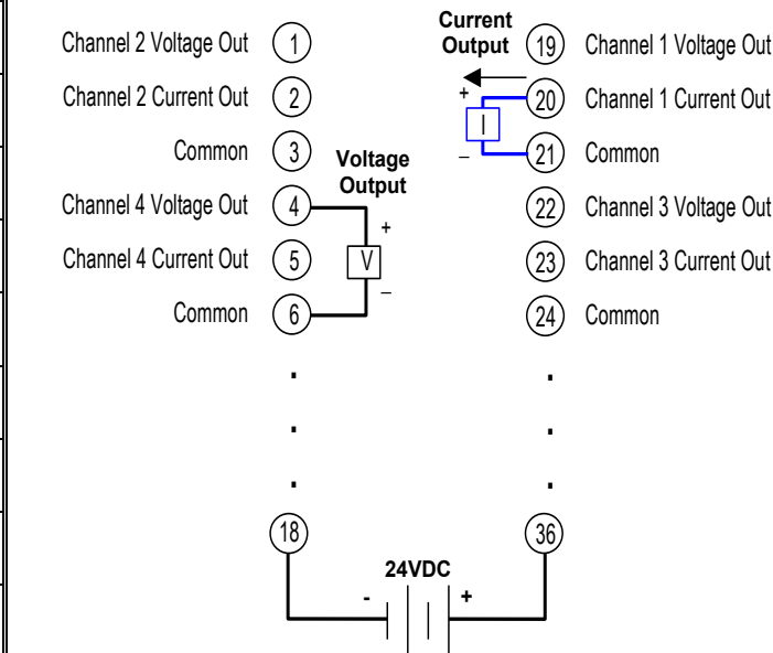
Figure 324: Field Wiring ALG728
