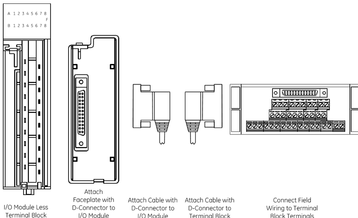
Figure 432: Low-Density Terminal Block Quick Connect System
