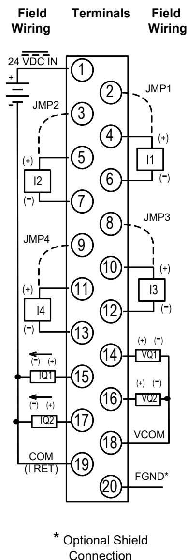
Figure 341: Field Wiring ALG542
