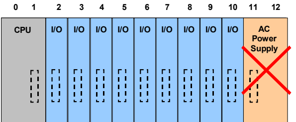
Figure 64: Invalid: AC Power Supply cannot be in Slot 11
