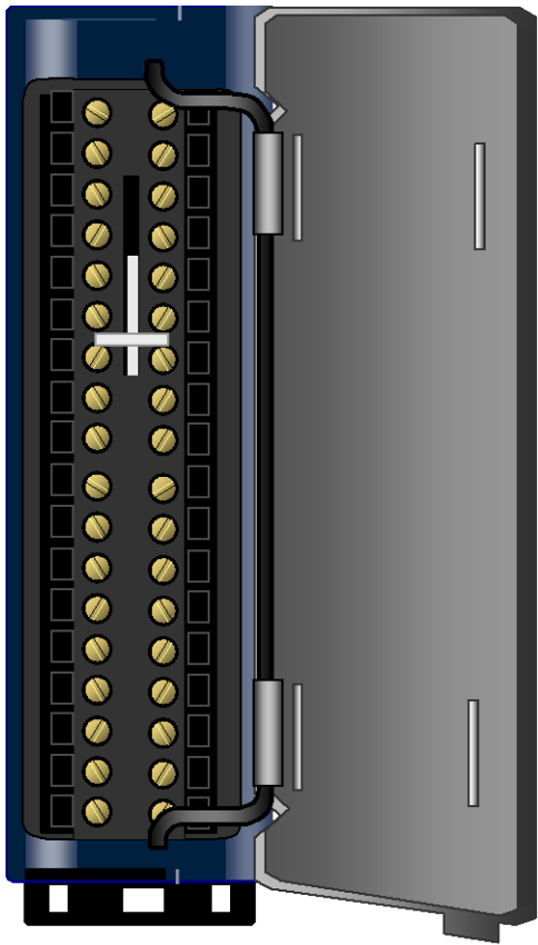
Figure 426: 36-Terminal Box-Style Terminal Block
