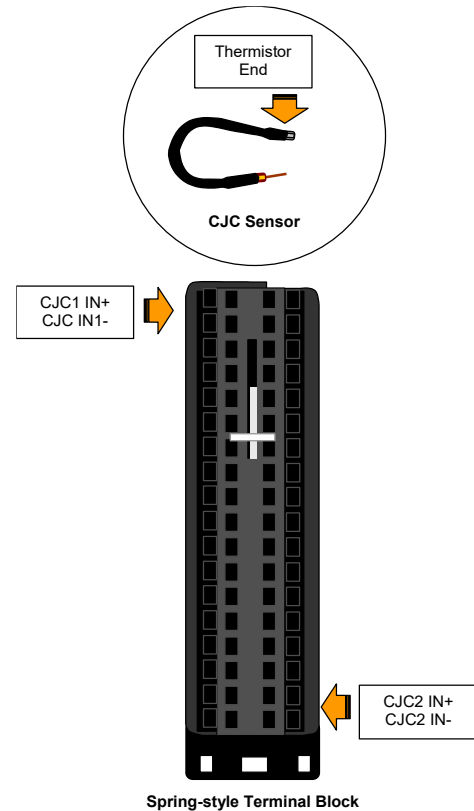
Figure 349: Installing Cold Junction Sensor
