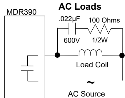
Figure 255: Suppression of AC Loads MDR390
