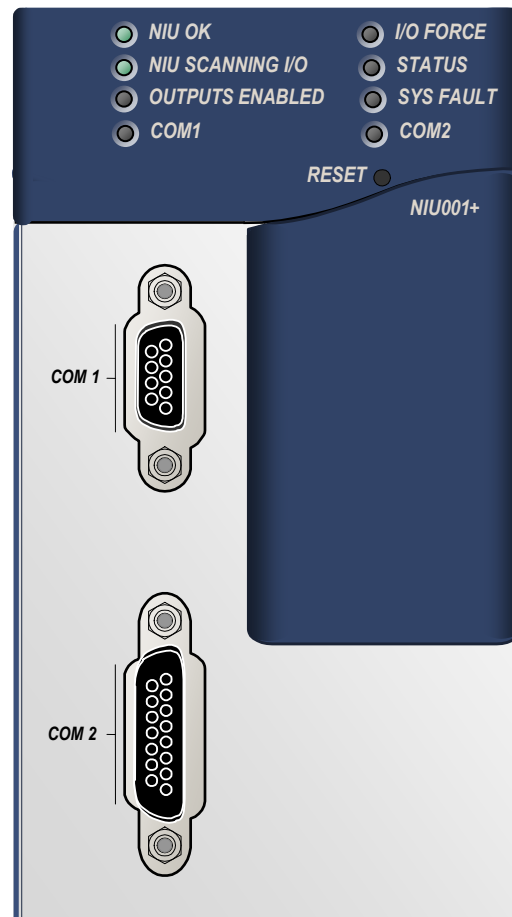
Figure 405: IC695NIU001 PLUS
