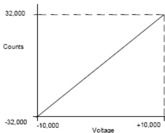
Figure 343: Output Scaling Example ALG542
