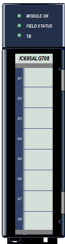
Figure 305: IC695ALG708
