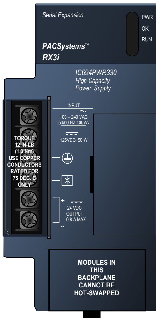
Figure 110: IC694PWR330
