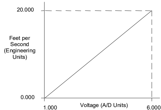
Figure 350: Input Scaling Example 1: ALG600
