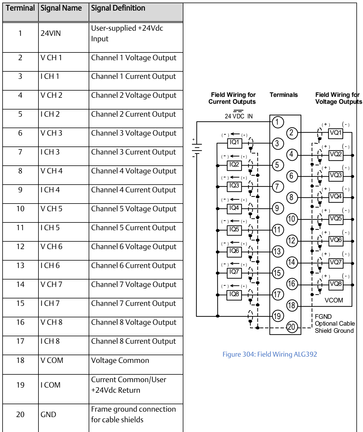
Figure 304 shows connections for current and voltage outputs. Each channel can be configured to operate as a voltage output or a current output - not both simultaneously.
