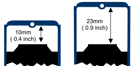
Figure 425: Depth Comparison: High-Density vs Extended High-Density Terminal Block
