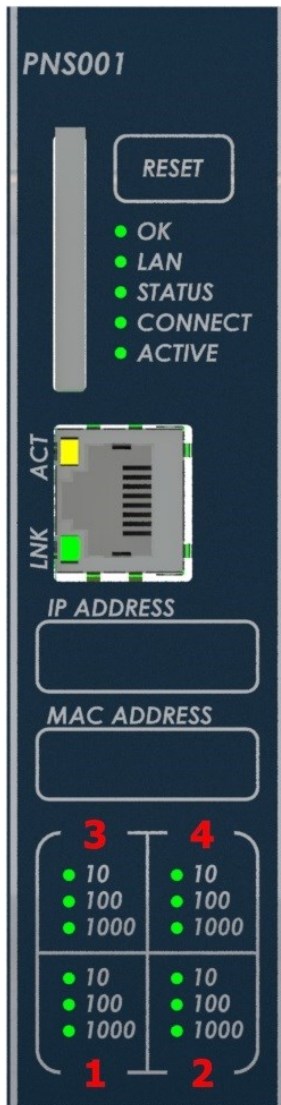
Figure 409: IC695PNS001-Bxxx
