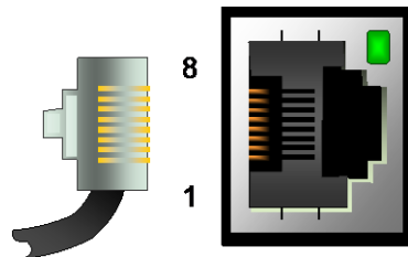
Figure 421: RJ-45 Pinout PRS015
