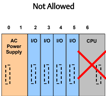
Figure 70: CPU cannot be configured in Slot 6
