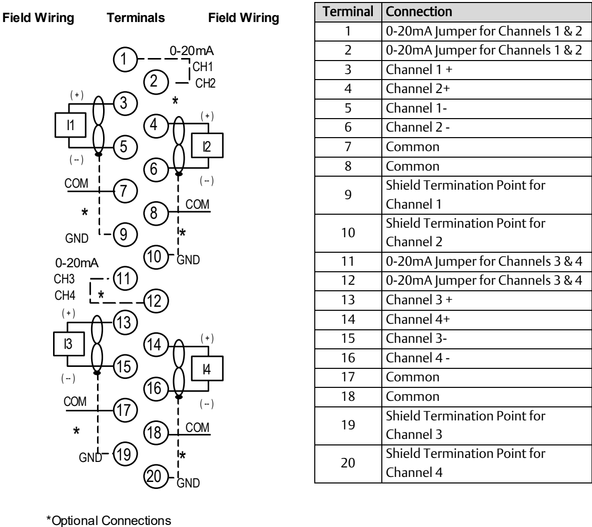
Figure 266: Field Wiring ALG221
