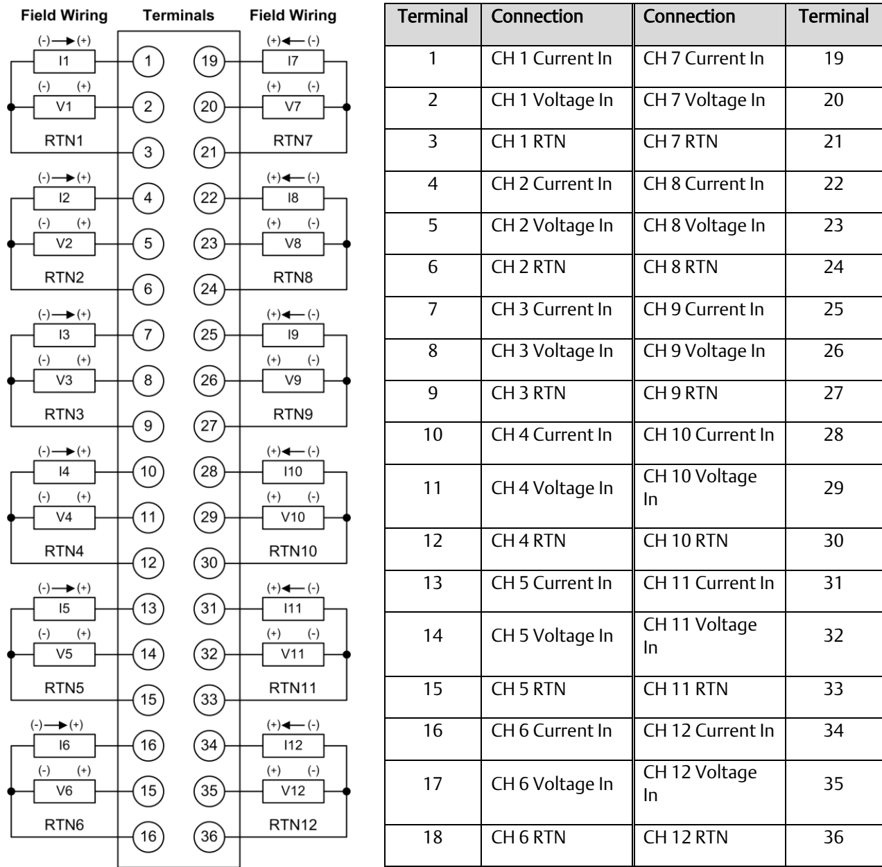
Figure 259: Field Wiring: ALG112
