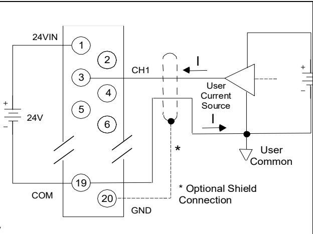
Figure 275: Connection Example 2 ALG222
