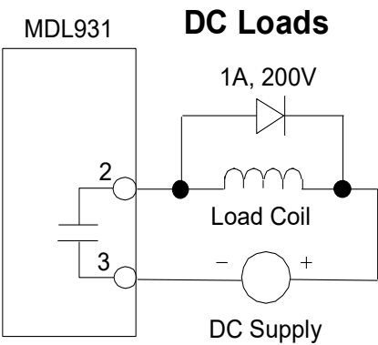
Figure 234: Suppression of DC Loads MDL931
