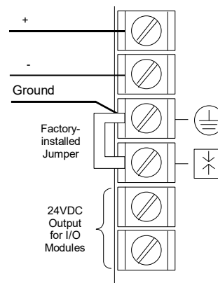
Figure 115: Field Wiring for PWR331
