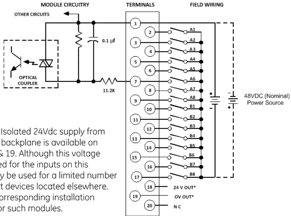
Figure 154: Field Wiring MDL648
