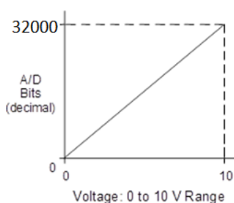
Figure 277: Input Scaling ALG232
