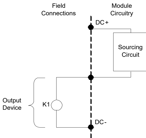
Figure 220: Circuit Detail MDL765
