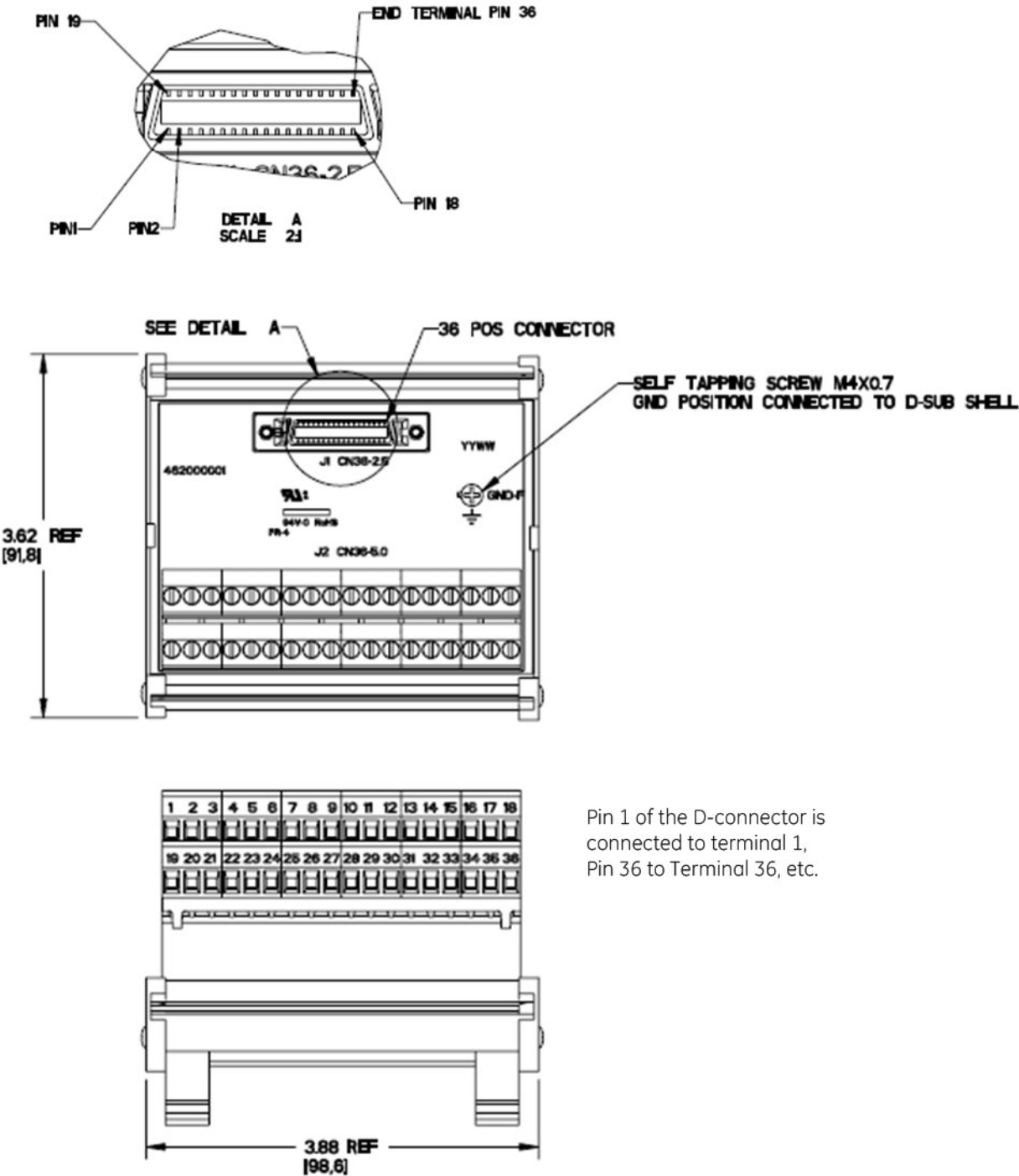
Figure 450: IC694RTB032 High-Density Remote Base, 36-Terminal
