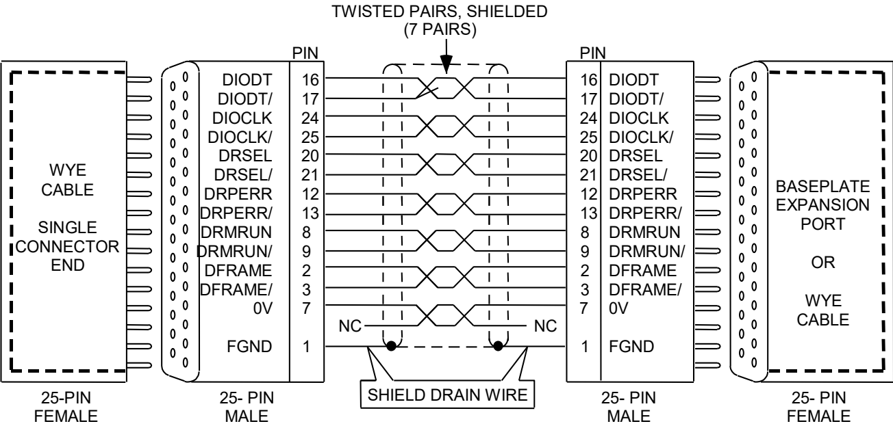
Figure 125: Wiring Diagram – Cable without Continuous Shielding
