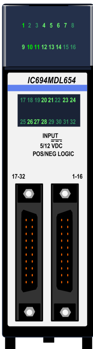
Figure 155: IC694MDL654
