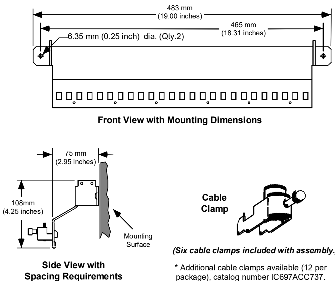
Figure 455: Cable Clamp IC697ACC736 Diagrams
