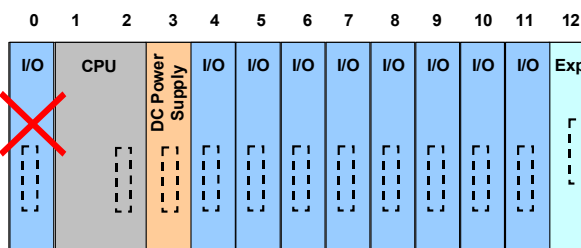
Figure 68: Invalid: Only a Power Supply can be installed in Slot
