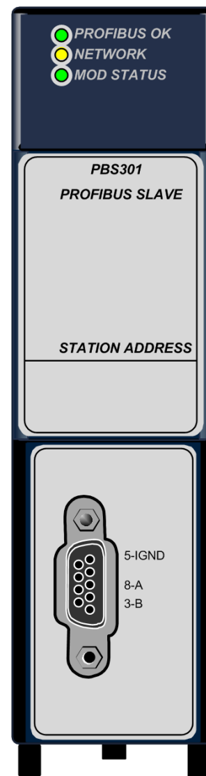
Figure 407: IC695PBS301
