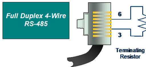
Figure 422: Externally-Mounted Terminating Resistor
