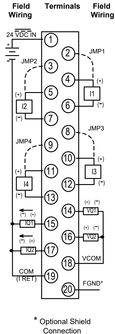
Figure 341: Field Wiring ALG542
