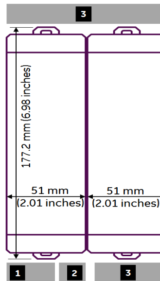
Figure 411: Mounting Diagram CEP001 & CEE001
