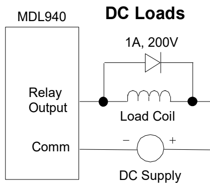
Figure 238: Suppression of DC Loads MDL940
