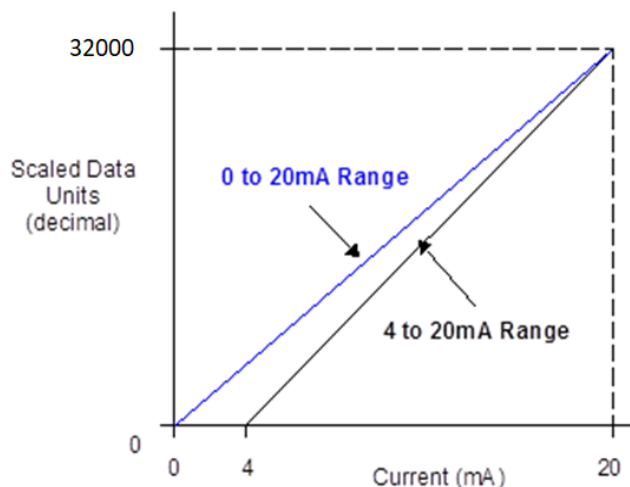
Figure 282: Input Scaling ALG233
