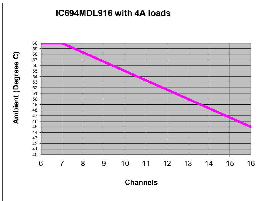
Figure 222: Thermal Derating Curve MDL916
