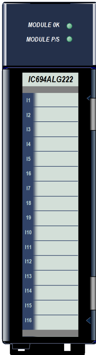
Figure 267: IC694ALG222
