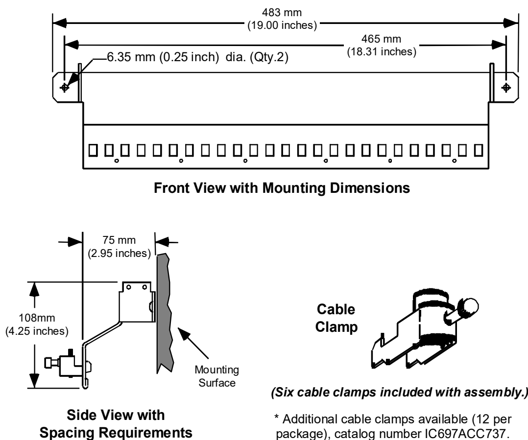
Figure 455: Cable Clamp IC697ACC736 Diagrams
