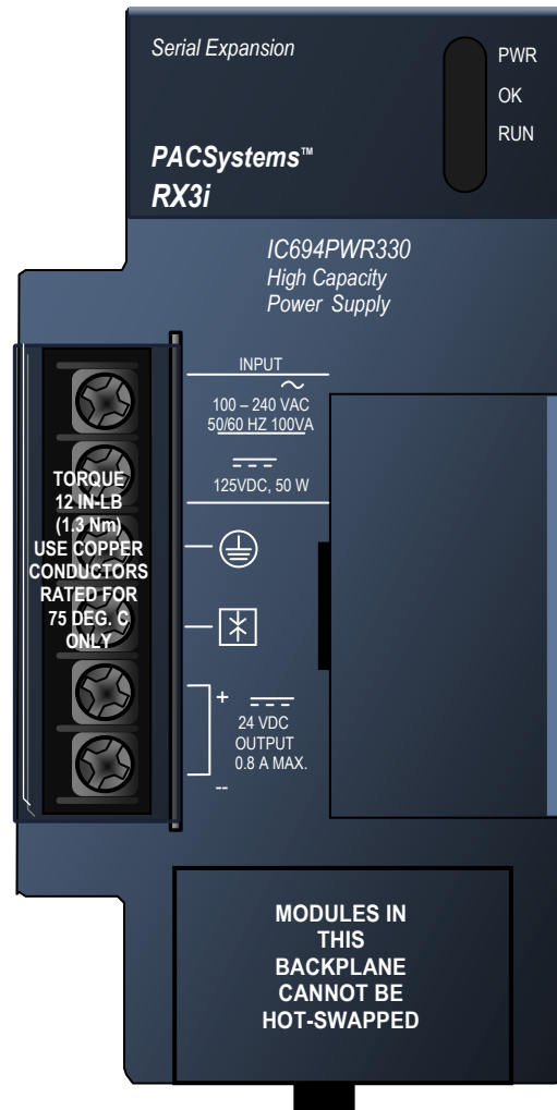
Figure 110: IC694PWR330
