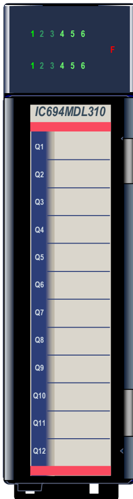
Figure 174: IC694MDL310
