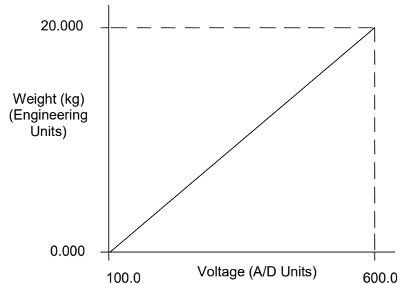
Figure 360: Input Scaling Example ALG508
