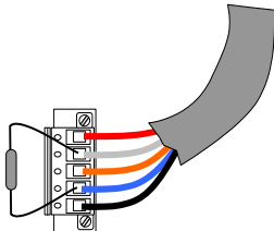
Figure 385: DeviceNet Terminating Resistor Installation
