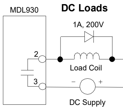
Figure 229: Suppression of DC Loads MDL930
