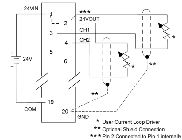
Figure 284: Connection Example 1 ALG233
