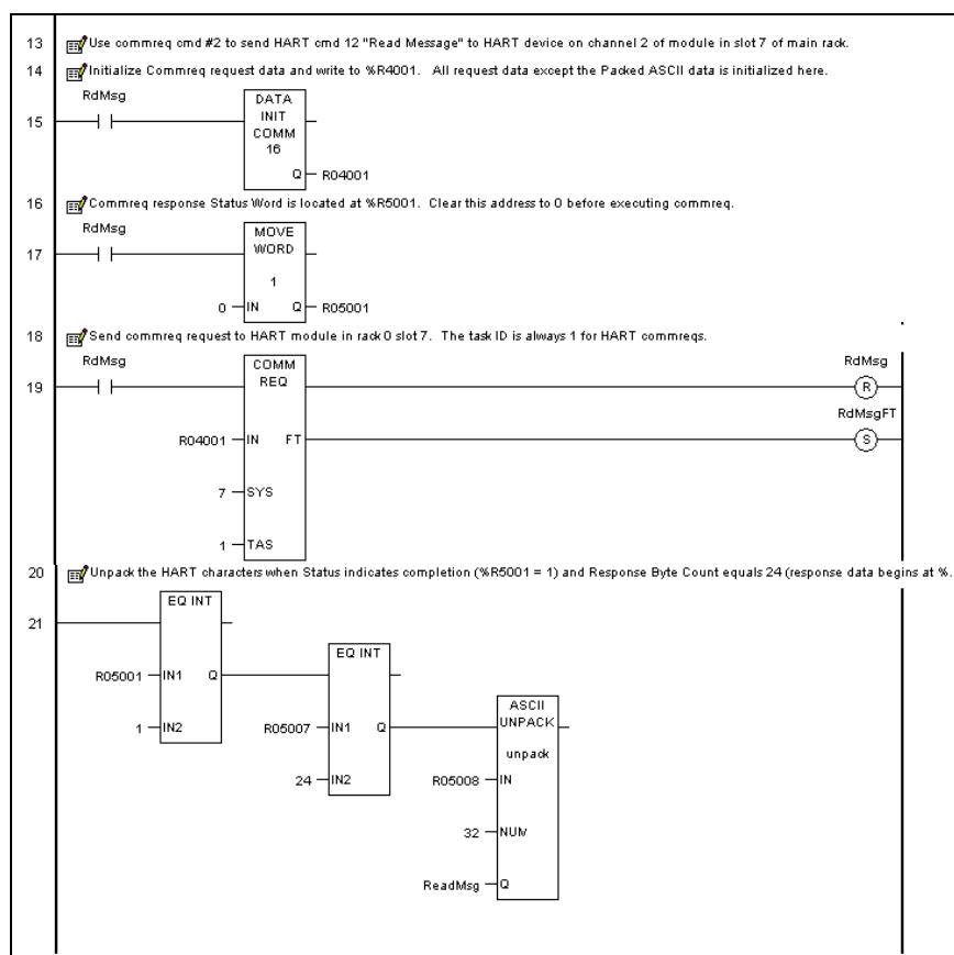
Figure 330: Ladder Logic for ACSII Unpack
