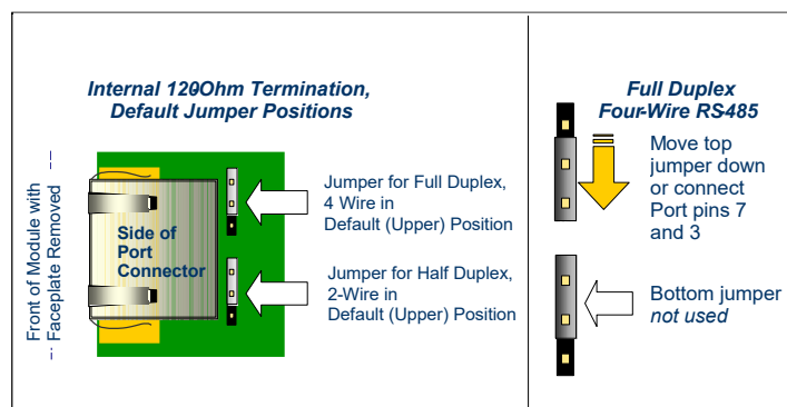
Figure 423: Using the Internal Terminating Resistor PRS015
