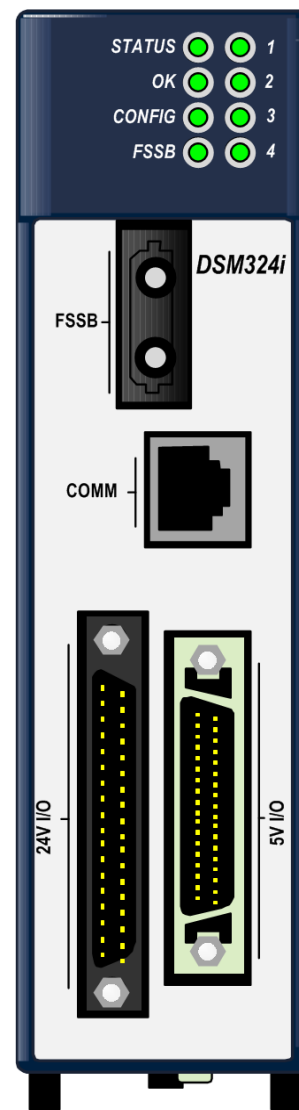
Figure 393: DSM324 Features
