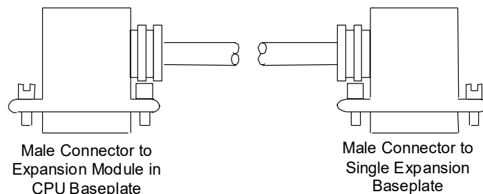
Figure 119: Cable IC693CBL302
