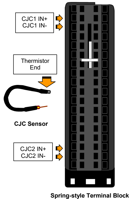
Figure 355: Installing Cold Junction Sensor
