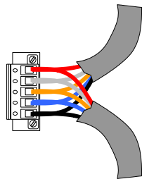
Figure 387: DeviceNet Wiring for Daisy Chain
