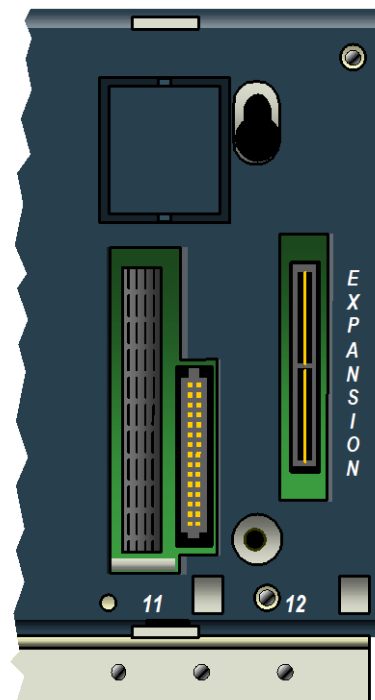
Figure 61: Expansion Slot Connector is shown at Slot 12
