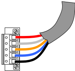
Figure 386: DeviceNet Wiring for End of Segment
