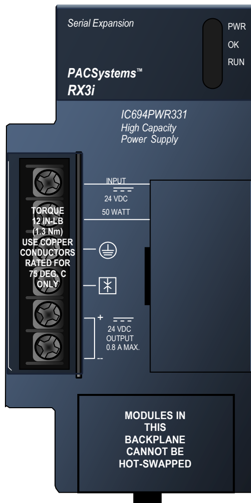
Figure 113: IC694PWR331
