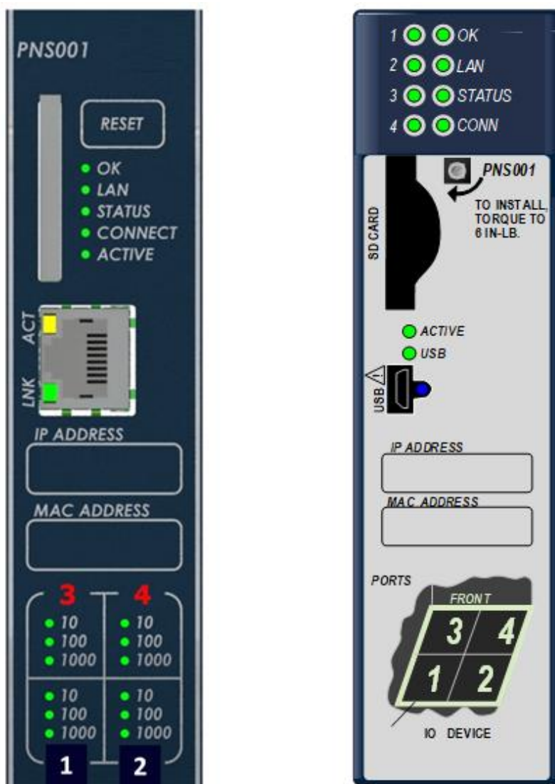
Figure 4: IC695PNS001-Bxxx (left) and IC695PNS001-Axxx (right) LEDs
