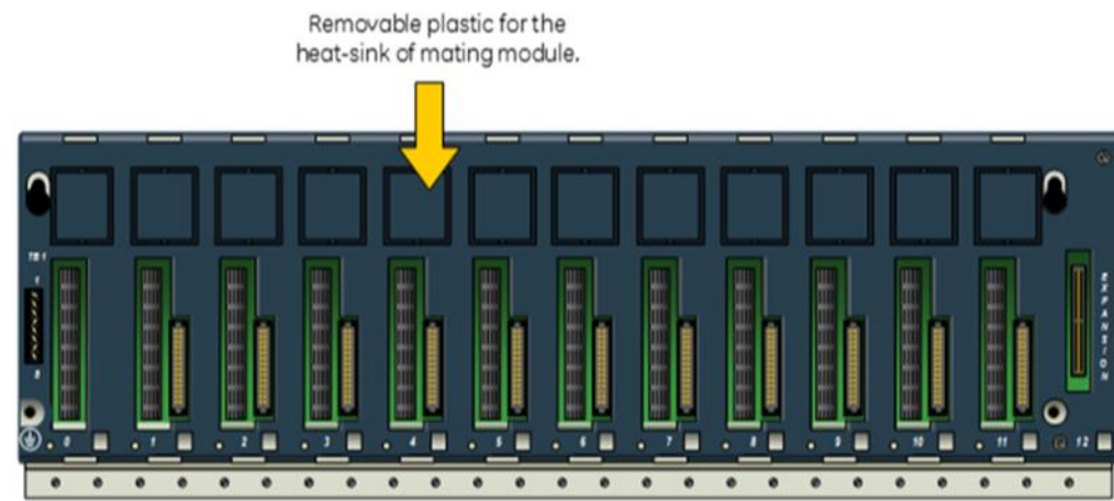
Figure 7: RX3i Backplane showing Removable Plastic Knockout
