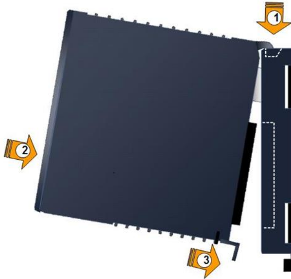
Figure 8: Install Module into RX3i Backplane Backplane
