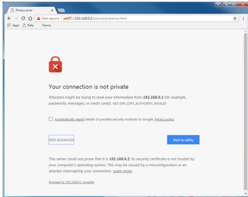
Figure 11: Privacy Warning
