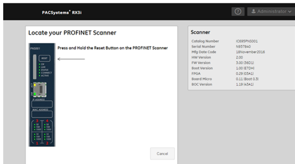
Figure 12: Locate Device
