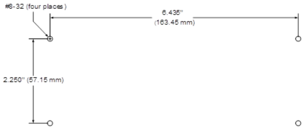
Figure 3: Mounting Diagram for IC690RBT001 Rechargeable Battery
