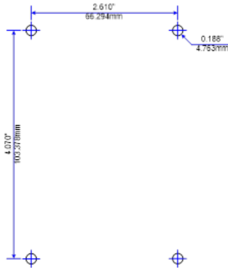
Figure 8: Drilling Pattern for Direct Panel Mounting
