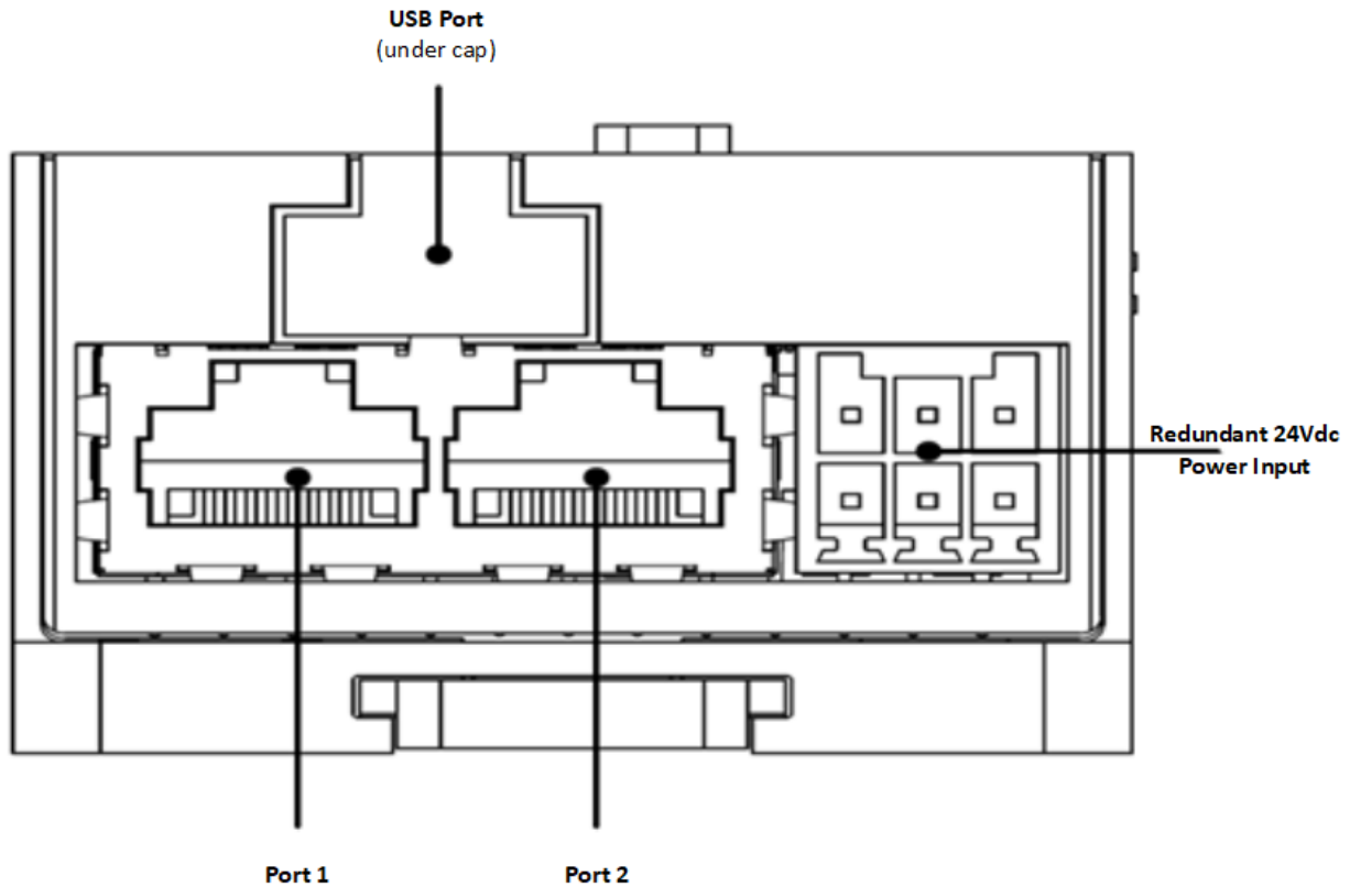
Figure 5: Underside of CEP001 Showing Ethernet Ports
