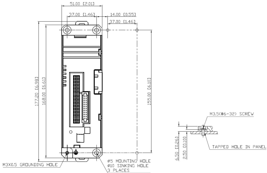
Figure 9: Panel Mount
