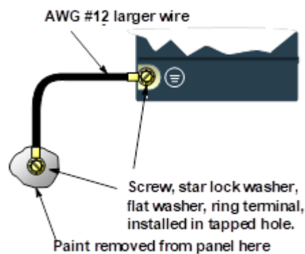
Figure 11: Grounding Diagram
