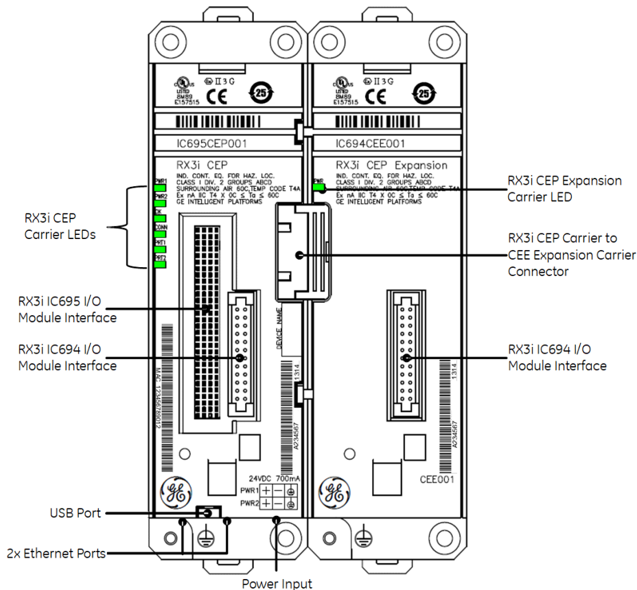
Figure 1: RX3i CEP Carrier with the Expansion Carrier Connected
