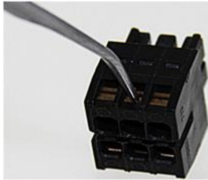
Figure 12: Spring Clamp Release
