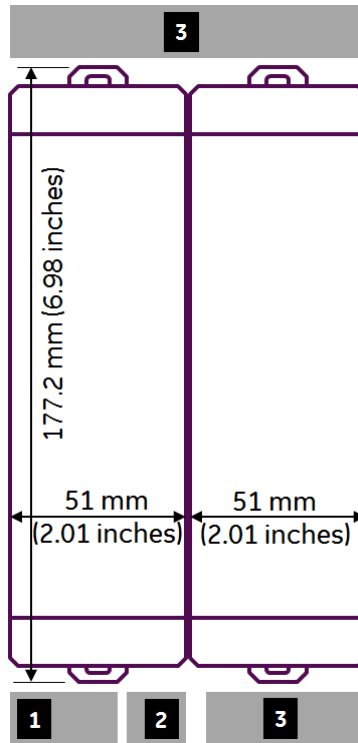
Figure 6: Mounting & Clearance Notes CEP001 & CEE001
