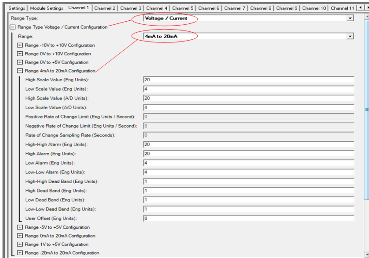
Figure 15: Configuration of Multiple Options for Certain IO Modules
