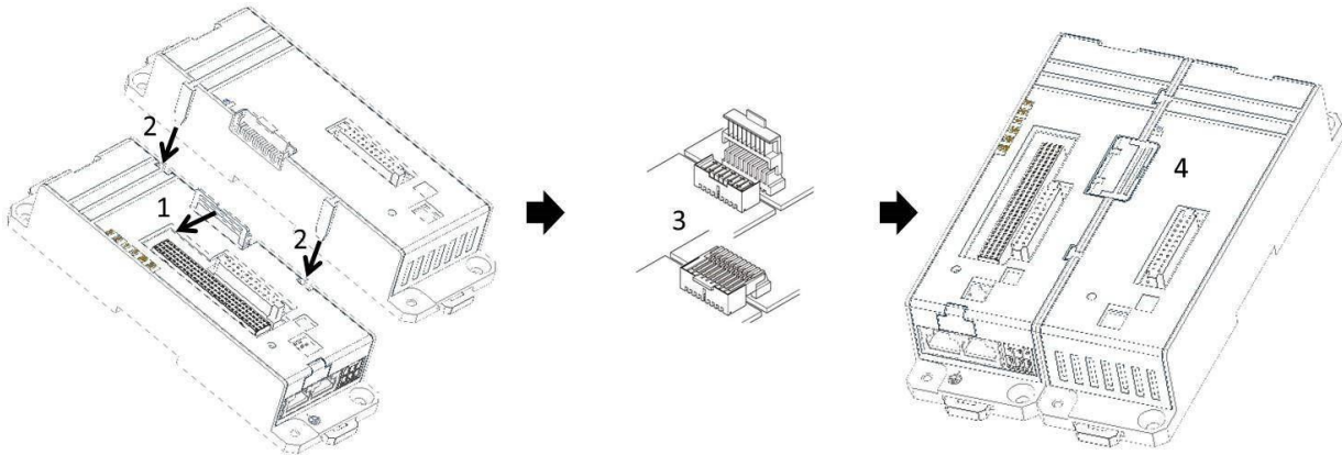
Figure 10: Interconnecting CEP001 & CEE001
